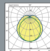
MONO LED BAR 48W 6800lm
